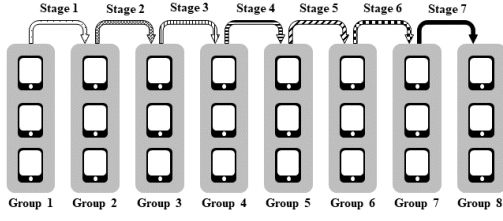
(a) Turbo-Aggregate. Each arrow is carried out sequentially. Turbo-Aggregate requires 7 stages.
